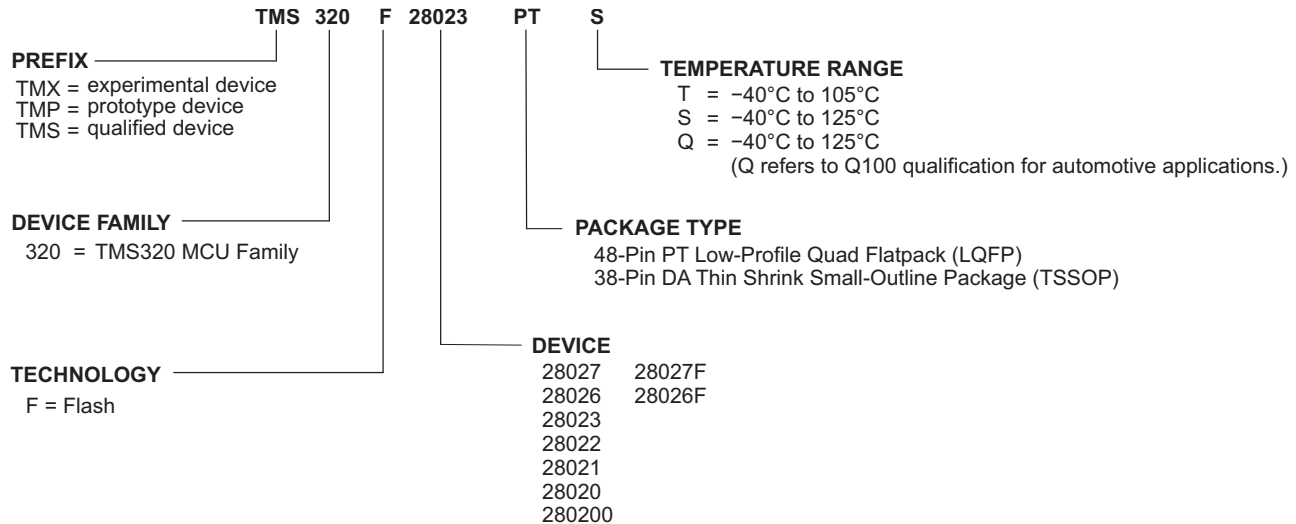
Figure 8-1. Device Nomenclature
