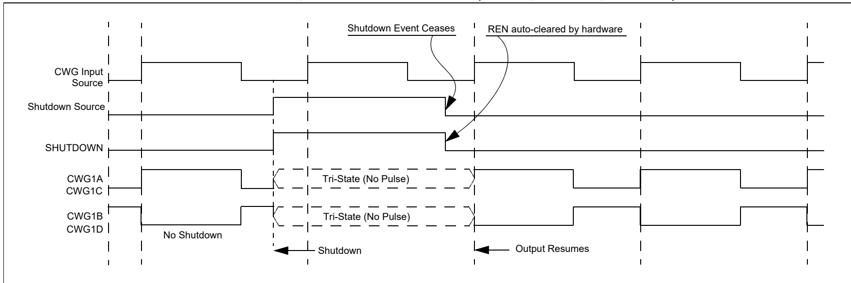
FIGURE 30-14: SHUTDOWN FUNCTIONALITY, AUTO-RESTART ENABLED (REN = 1, LSAC = 01, LSBSD = 01)
