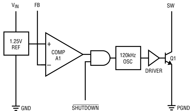
LT1109A (Adjustable)
