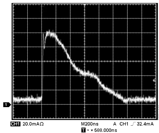
Figure 28. OTP Program Energy Plot for Single Fuse
