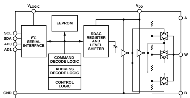
Figure 2. Block Diagram Showing Level Shifters
