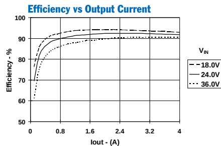
PT6886, V_{out} = 12V (Note A)
