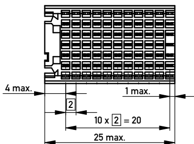
CONTACT LAYOUT
