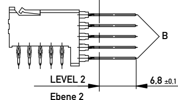
DATUM PLANE DEPTH
