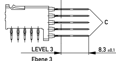
DATUM PLANE DEPTH
