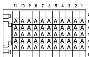
CONTACT LAYOUT
