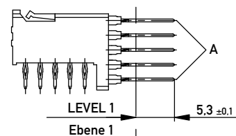
CONTACT LENGTH EXAMPLES
