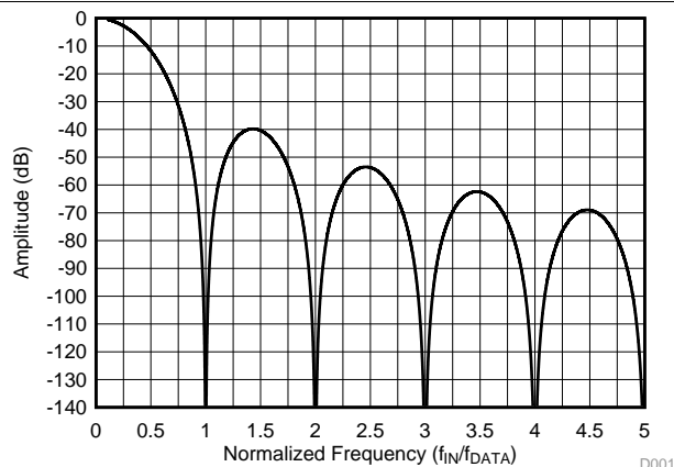
Figure 45. Sinc³ Filter Frequency Response
