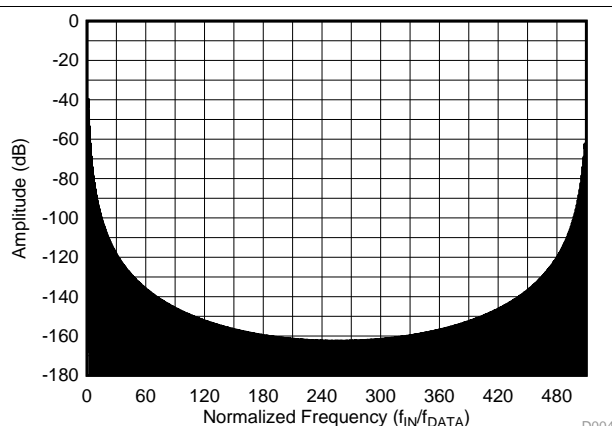
Figure 48. Sinc³ Filter Frequency Response (OSR 512)
