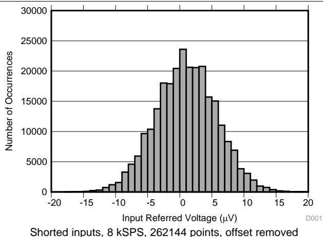
Figure 10. Single Device Noise Histogram
