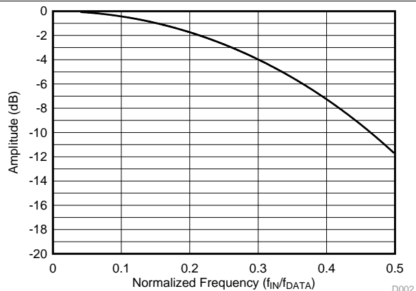
Figure 46. Sinc³ Filter Roll-Off
