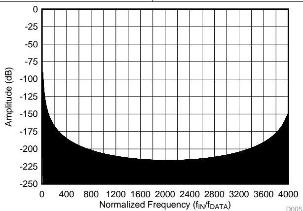
Figure 49. Sinc³ Filter Frequency Response (OSR 4096)
