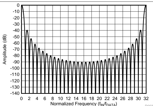
Figure 47. Sinc³ Filter Frequency Response (OSR 32)
