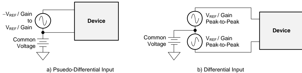
Figure 39. Pseudo-Differential and Fully-Differential Inputs
