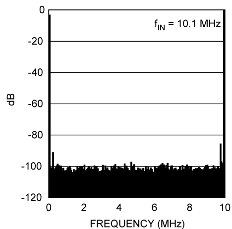
Spectral Response, 10.1 MHz Input
