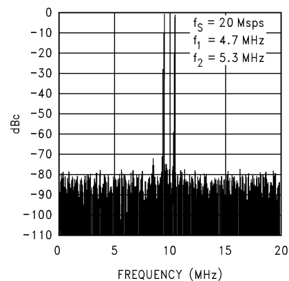
IMD @ F_1 = 9.5\text{ MHz} , F_2 = 10.5\text{ MHz}
