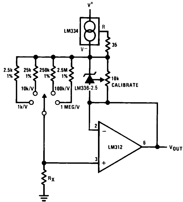
Linear Ohmmeter
