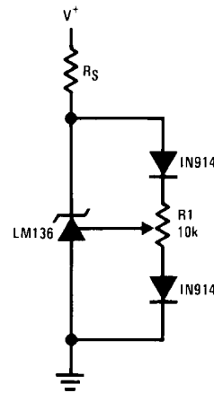
FIGURE 1. LM136 With Pot for Adjustment of Breakdown Voltage (Trim Range = \pm 120 mV typical)
