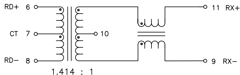
SCHEMATIC
