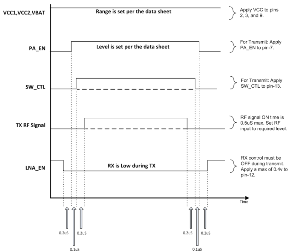
Transmit Timing Diagram Power ON / OFF Sequence
