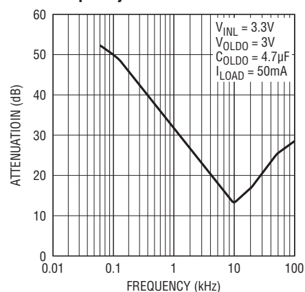
LDO Input Ripple Rejection vs Frequency
