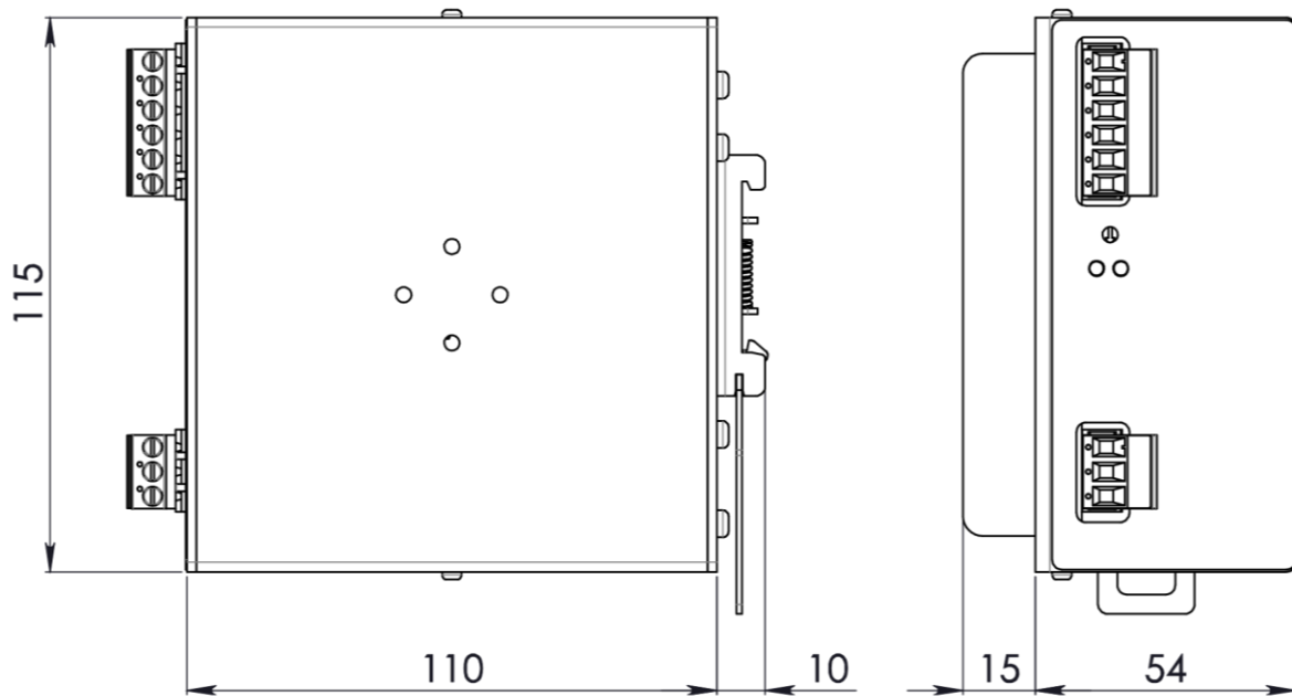
Figure 1. Mechanical Drawing
