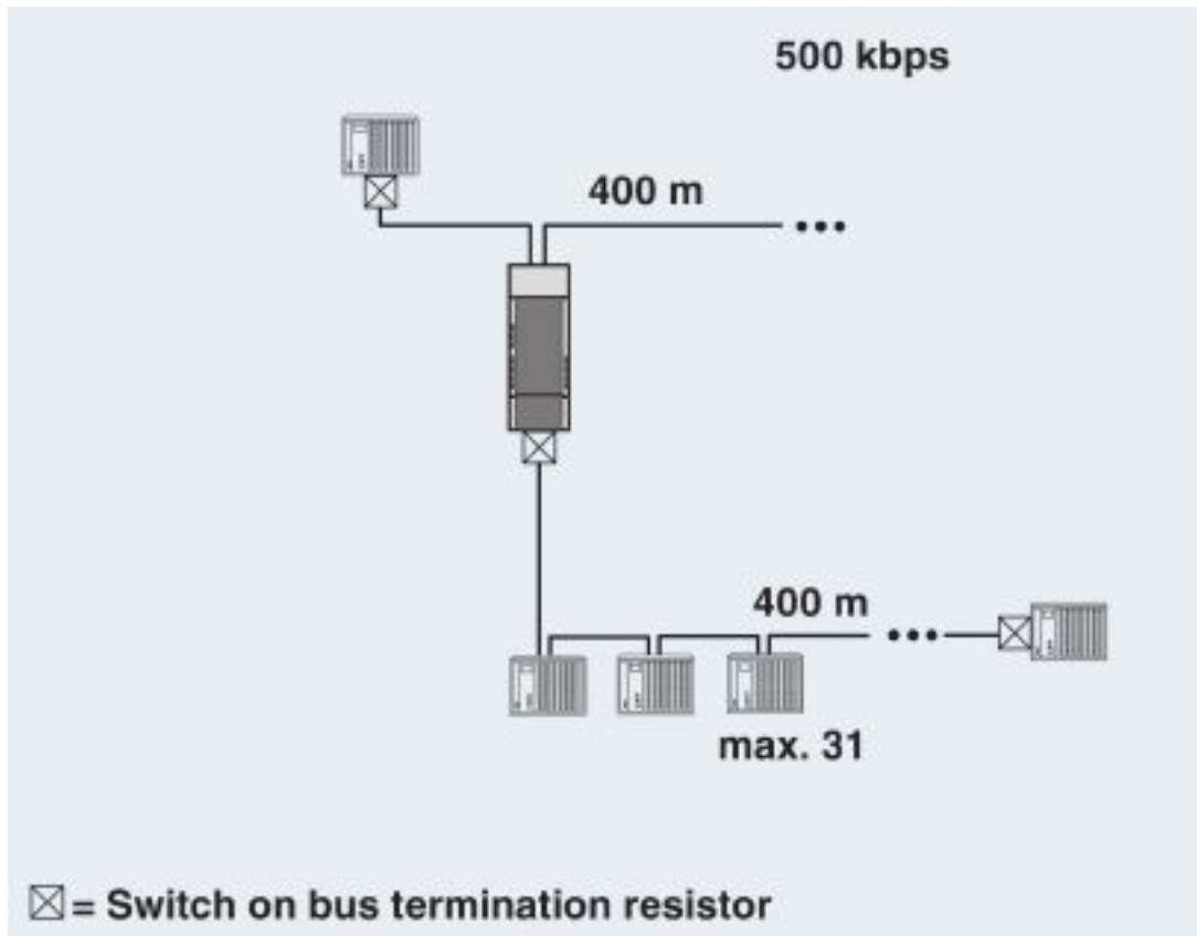
Branch/bus segmentation
