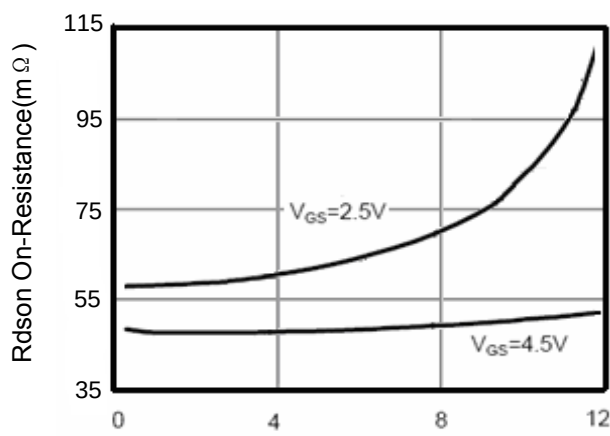
Figure 6 Drain-Source On-Resistance
