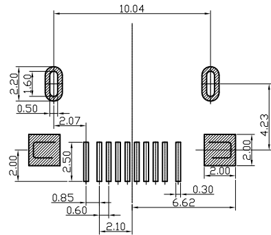
RECOMMENDED P.C.B LAYOUT(TOP VIEW) GENERAL TOLERANCE +/-0.05
