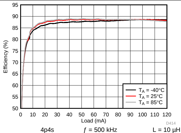
图 164. Backlight System Efficiency
