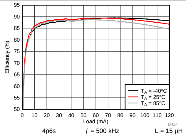
图 172. Backlight System Efficiency
