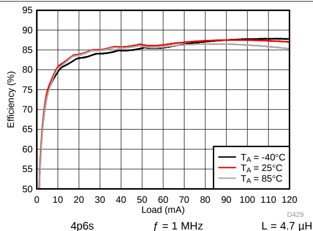
图 177. Backlight Boost Efficiency
