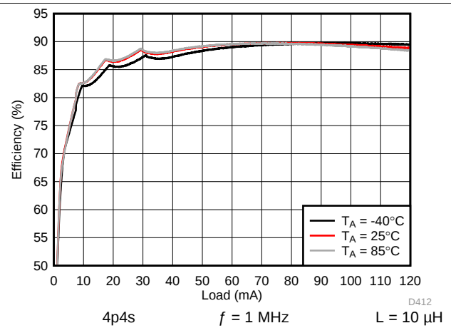
图 160. Backlight System Efficiency
