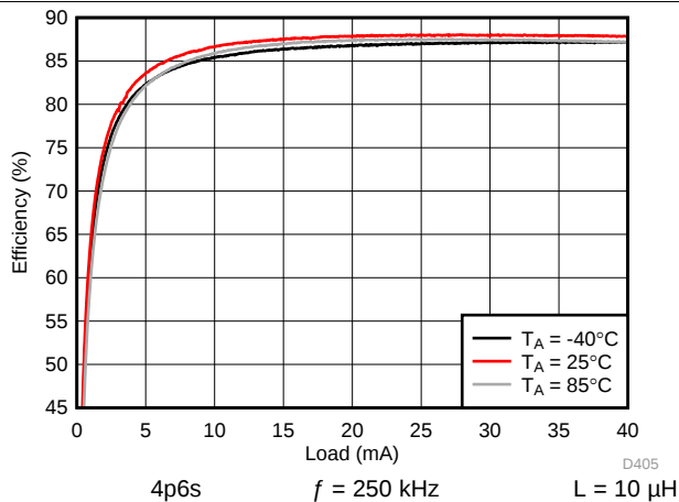
图 153. Backlight Boost Efficiency
