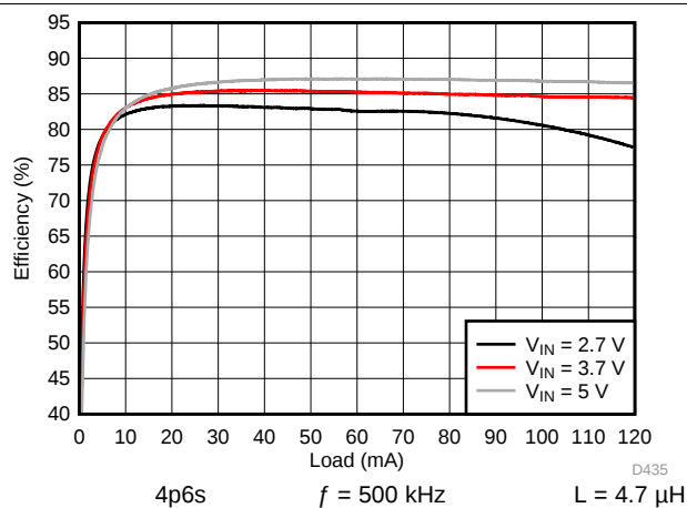
图 183. Backlight Boost Efficiency
