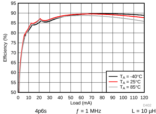
图 152. Backlight System Efficiency
