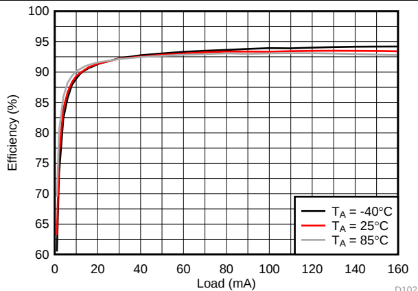
图 188. LCM Boost Efficiency
