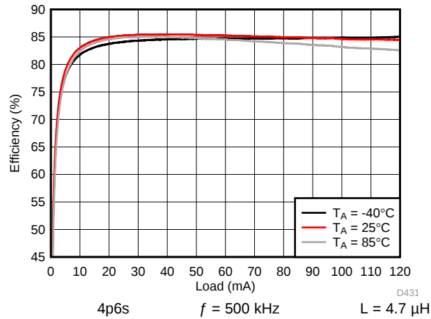
图 181. Backlight Boost Efficiency
