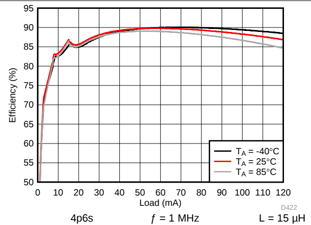
图 170. Backlight System Efficiency
