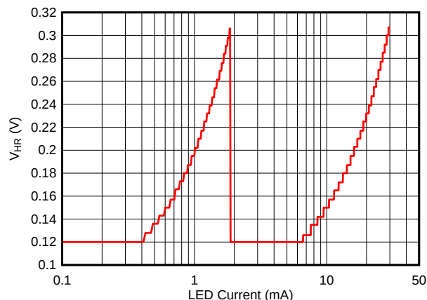
图 39. LM36274 Typical Exponential Regulated Headroom Voltage vs Programmed LED Current
