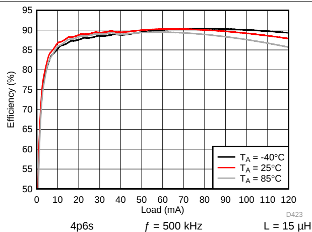
图 171. Backlight Boost Efficiency
