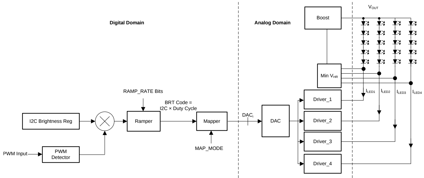
图 36. (I²C + PWM) Brightness Control, PWM Ramper Enabled
