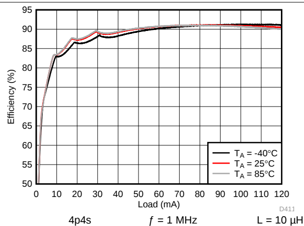
图 159. Backlight Boost Efficiency
