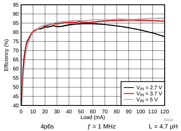
图 182. Backlight System Efficiency
