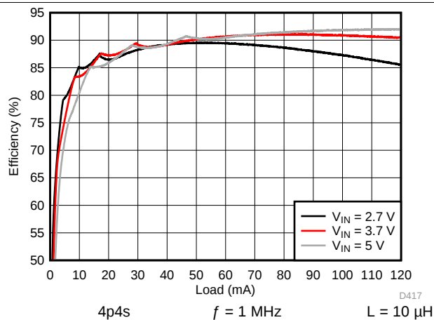
图 165. Backlight Boost Efficiency
