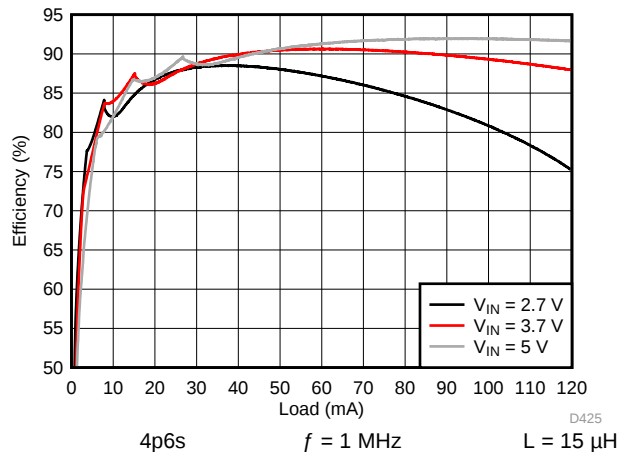
图 175. Backlight Boost Efficiency
