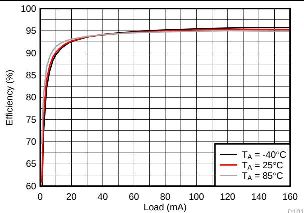
图 187. LCM Boost Efficiency
