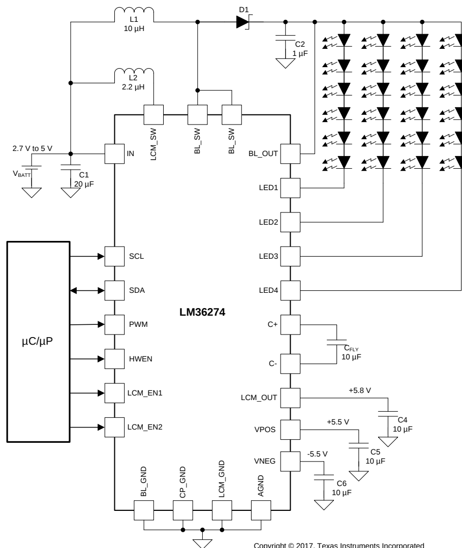
图 67. LM36274 Typical Application
