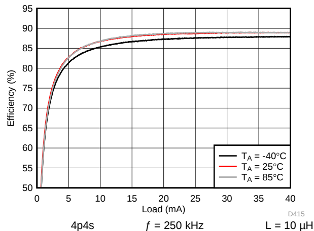
图 163. Backlight Boost Efficiency
