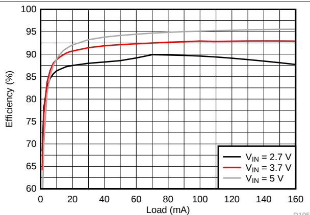
图 189. LCM Boost Efficiency
