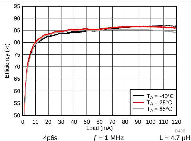
图 178. Backlight System Efficiency
