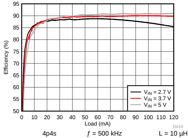
图 169. Backlight Boost Efficiency
