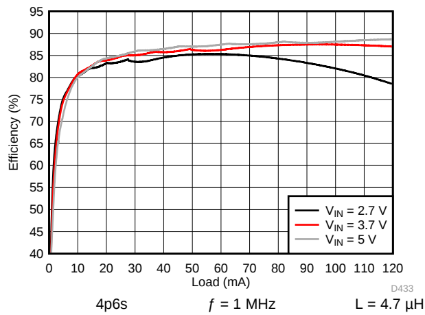
图 181. Backlight Boost Efficiency
