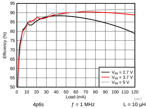
图 157. Backlight Boost Efficiency
