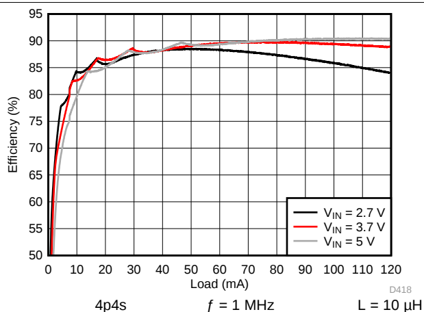
图 166. Backlight System Efficiency
