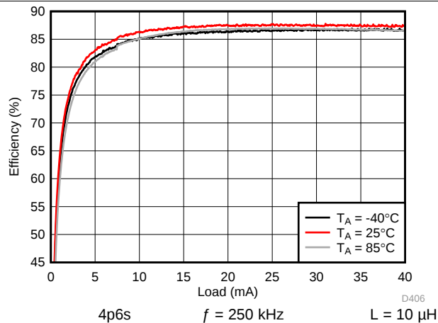
图 154. Backlight System Efficiency
