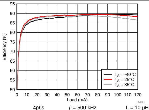
图 151. Backlight Boost Efficiency
