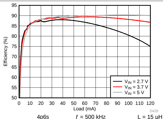
图 176. Backlight System Efficiency
