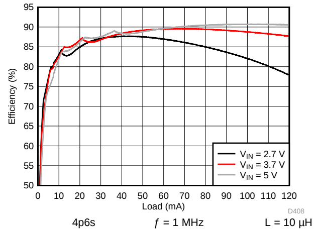
图 158. Backlight System Efficiency
