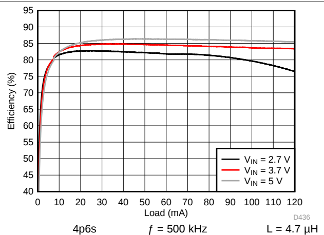
图 184. Backlight System Efficiency
