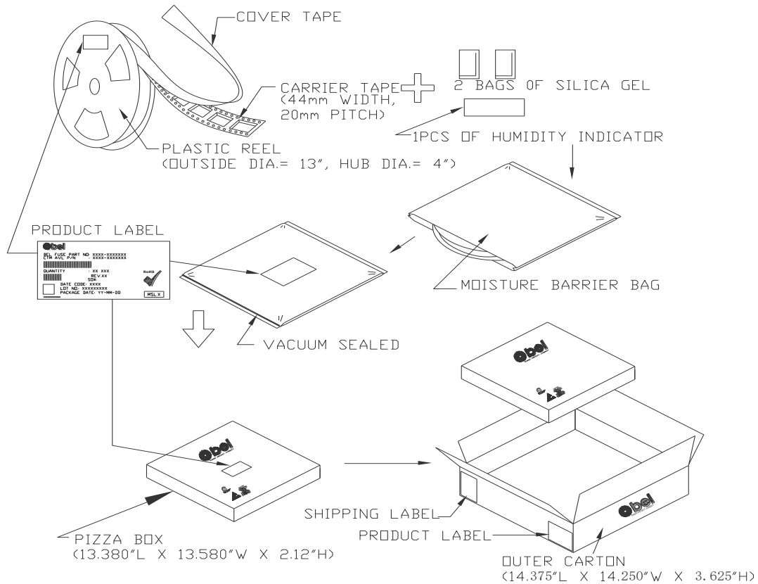
Figure 19. Packaging information-1
