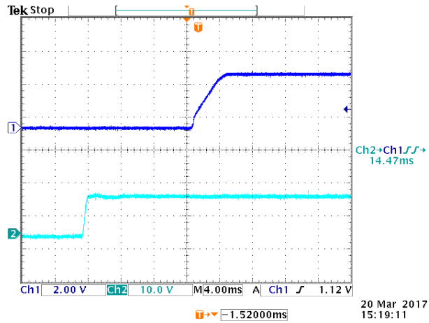
Figure 10. Startup
