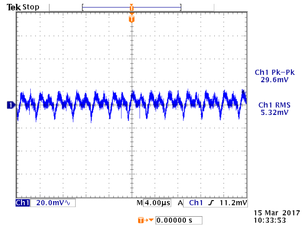
Figure 5. Ripple and noise at full load, V_{in} = 12\text{ V}
