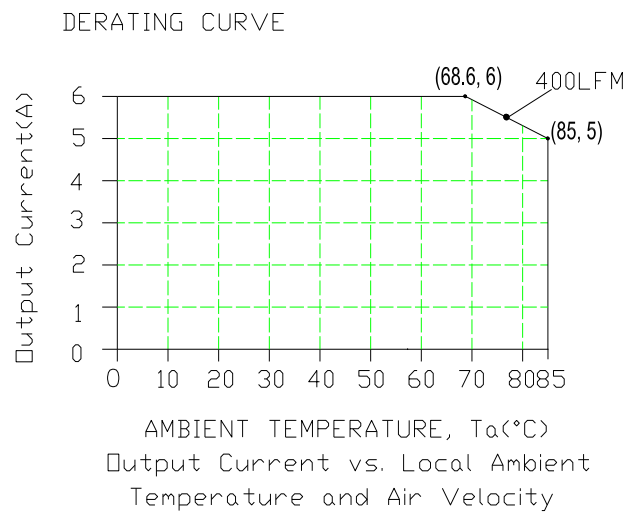
Figure 3. Thermal derating curve @ V in = 12 V, V o = 3.3 V
