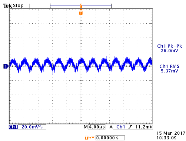
Figure 8. Ripple and noise at no load, V_{in} = 36\text{ V}
