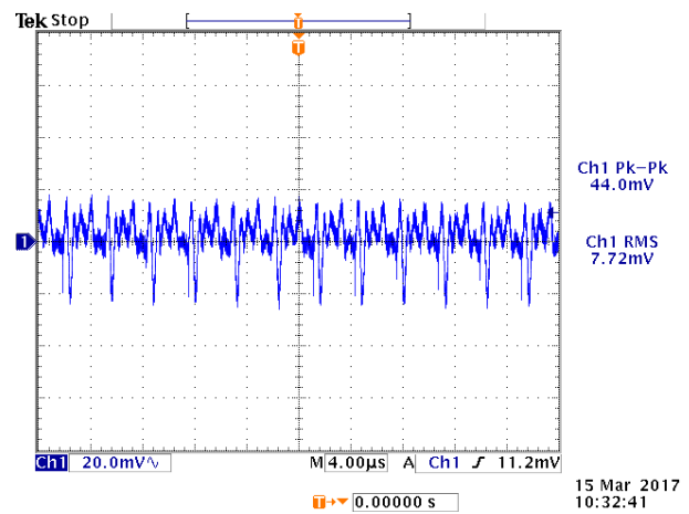
Figure 9. Ripple and noise at full load, V_{in} = 36\text{ V}
