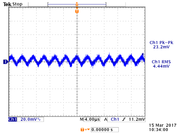
Figure 4. Ripple and noise at no load, V_{in} = 12\text{ V}
