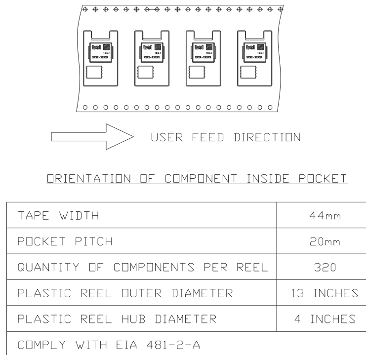
Figure 20. Packaging information-2
