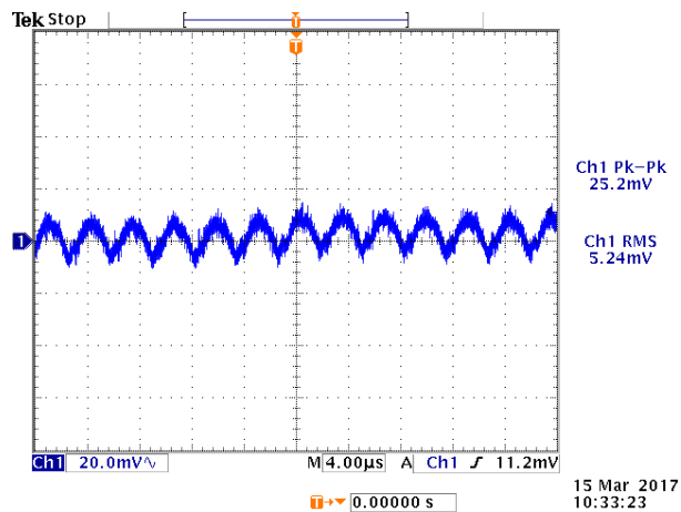
Figure 6. Ripple and noise at no load, V_{in} = 24\text{ V}
