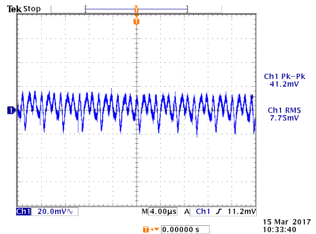
Figure 7. Ripple and noise at full load, V_{in} = 24\text{ V}
