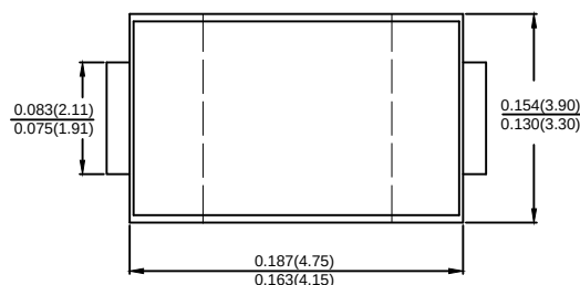
SMB/DO-214AA
