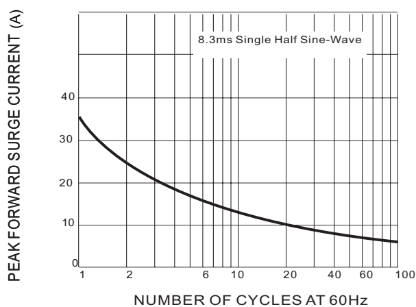
FIG.3 MAXIMUM NON-REPEITIVE SURGE CURRENT
