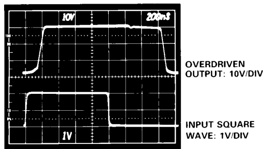
Figure 27. Overdrive Recovery
