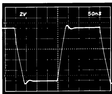
Figure 19b. Inverter Large Signal Pulse Response
