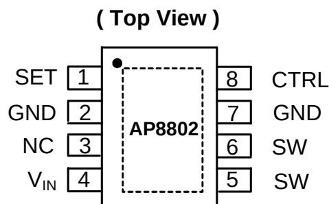
(2) SOP-8L-EP
