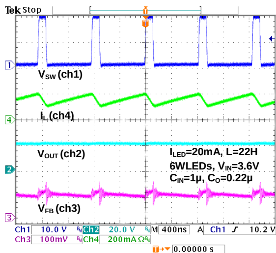
Figure 18. Operation Waveform
