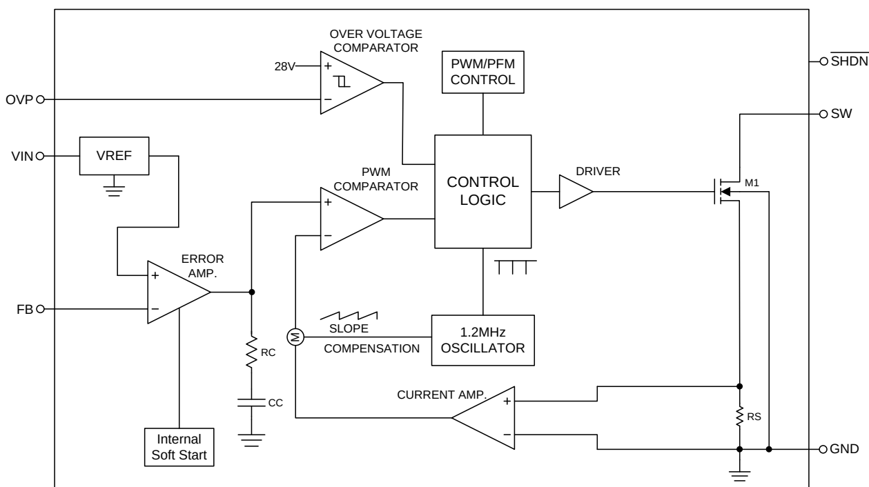
Figure 3. Block Diagram of FP6737/A
