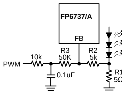
Figure 22. Dimming Control Using a Filtered PWM Signal
