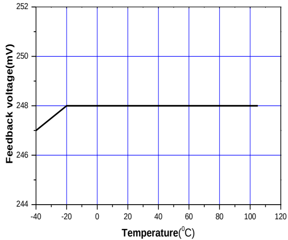
Figure 10. Feedback Voltage vs. Temperature
