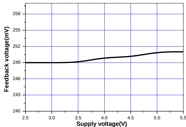
Figure 7. Feedback Voltage vs. Supply Voltage
