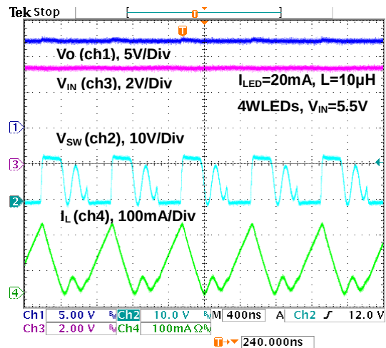
Figure 17. Operation Waveform
