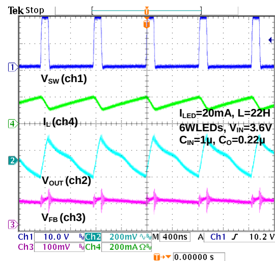
Figure 19. Operation Waveform
