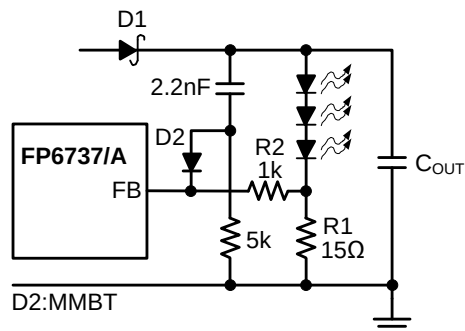
Figure 24. Recommended Soft-Startup Circuit
