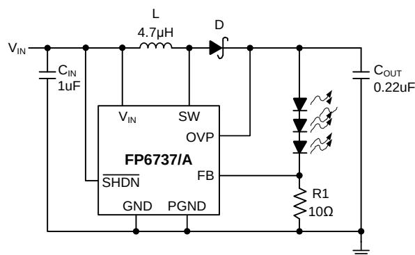
Figure 20. LED Driver with Open-Circuit Protection
