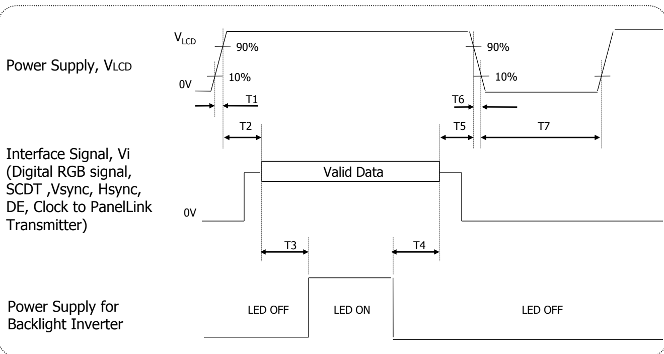
FIG.5 Power sequence
