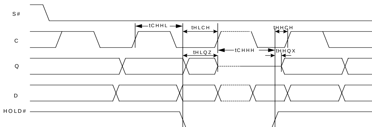
Figure 7: Hold Timing
