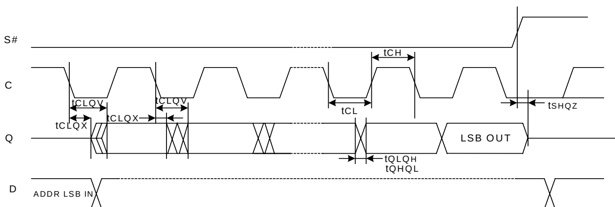
Figure 8: Output Timing
