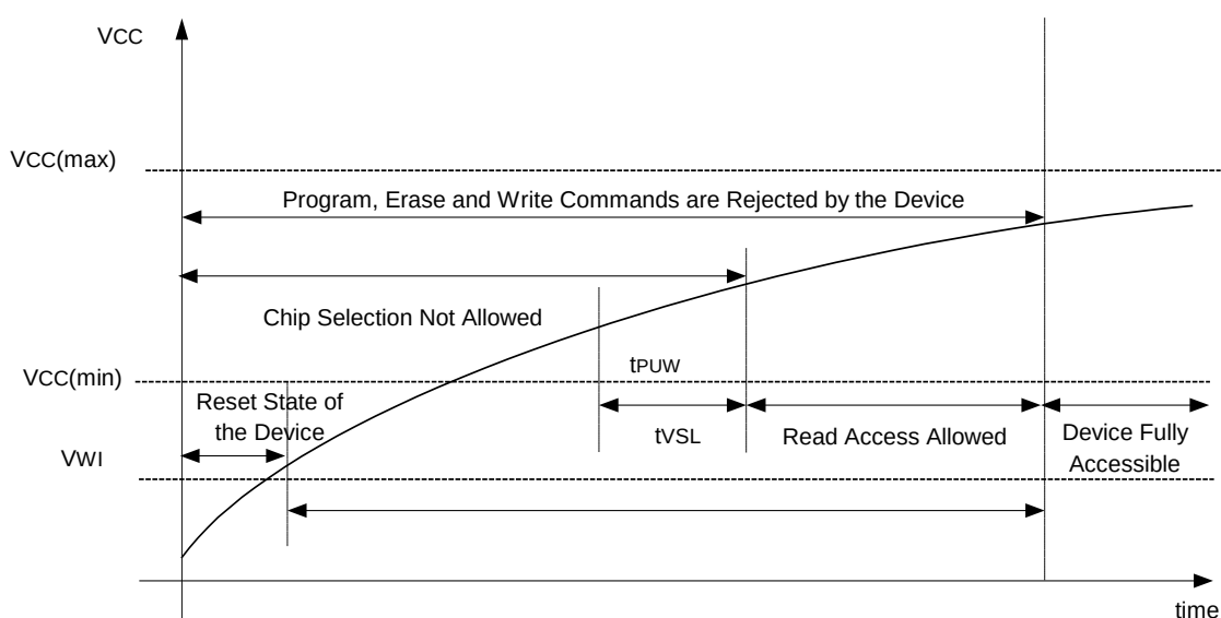
Figure 4: Power-up Timing
