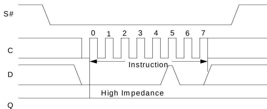
Figure 11: Write Disable (WRDI) Sequence
