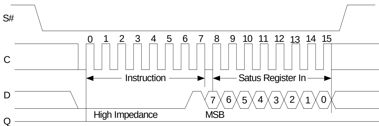
Figure 13: Write Status Register (WRSR) Sequence
