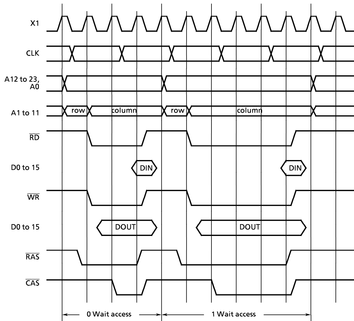
Figure 3.7 (3) DRAM Access Timing (Nomal Access Mode)
