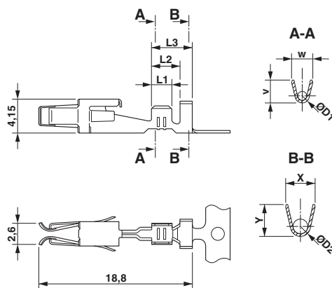
Dimensioned drawing
