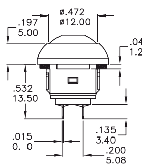
PB162B1TS1... ON-MOM Flat Top Actuator Snap-in Bushing Solder Lug Terminals IP67 for Panel Surface
