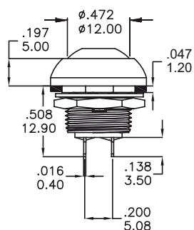
PB161B2TS1... OFF-MOM Flat Top Actuator Threaded Bushing Solder Lug Terminals IP67 for Panel Surface
