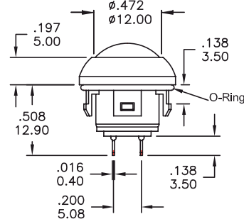
PB161RB3TS1... OFF-MOM Spherical Top Actuator Snap-in Bushing Solder Lug Terminals IP67 for Panel Surface
