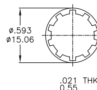
Locking Washer
