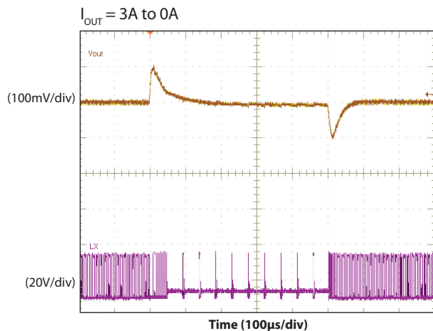
Transient Response
