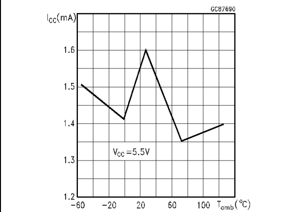
Figure 7. Driver short circuit supply current vs. temperature
