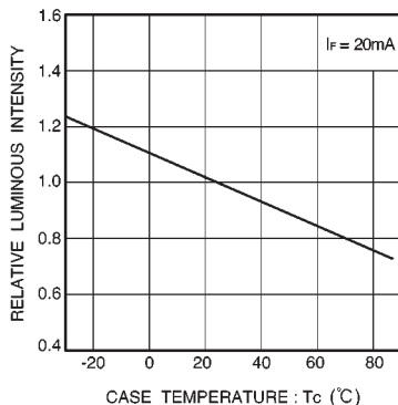
Fig. 15 Luminous intensity vs. case temperature
