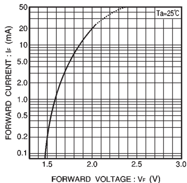
Fig. 14 Forward current vs. forward voltage
