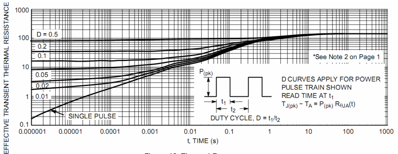
Figure 12. Thermal Response
