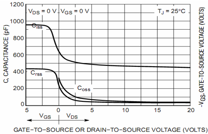
Figure 7. Capacitance Variation
