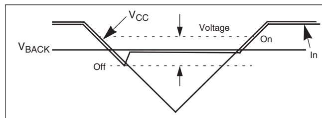
Figure 2. Power Control
