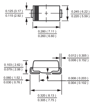
DO-214AB
