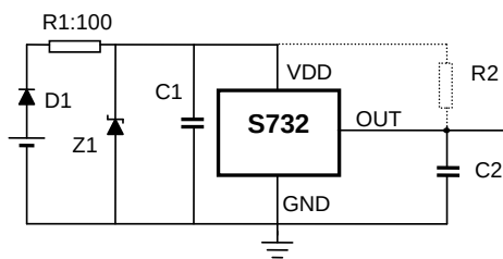
Automotive and Severe Environment Protection Circuit
