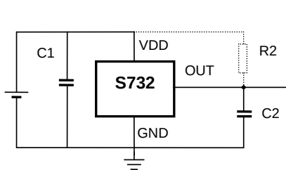
Typical Three-Wire Application Circuit
