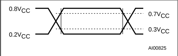
Figure 10. AC Testing Input Output Waveforms
