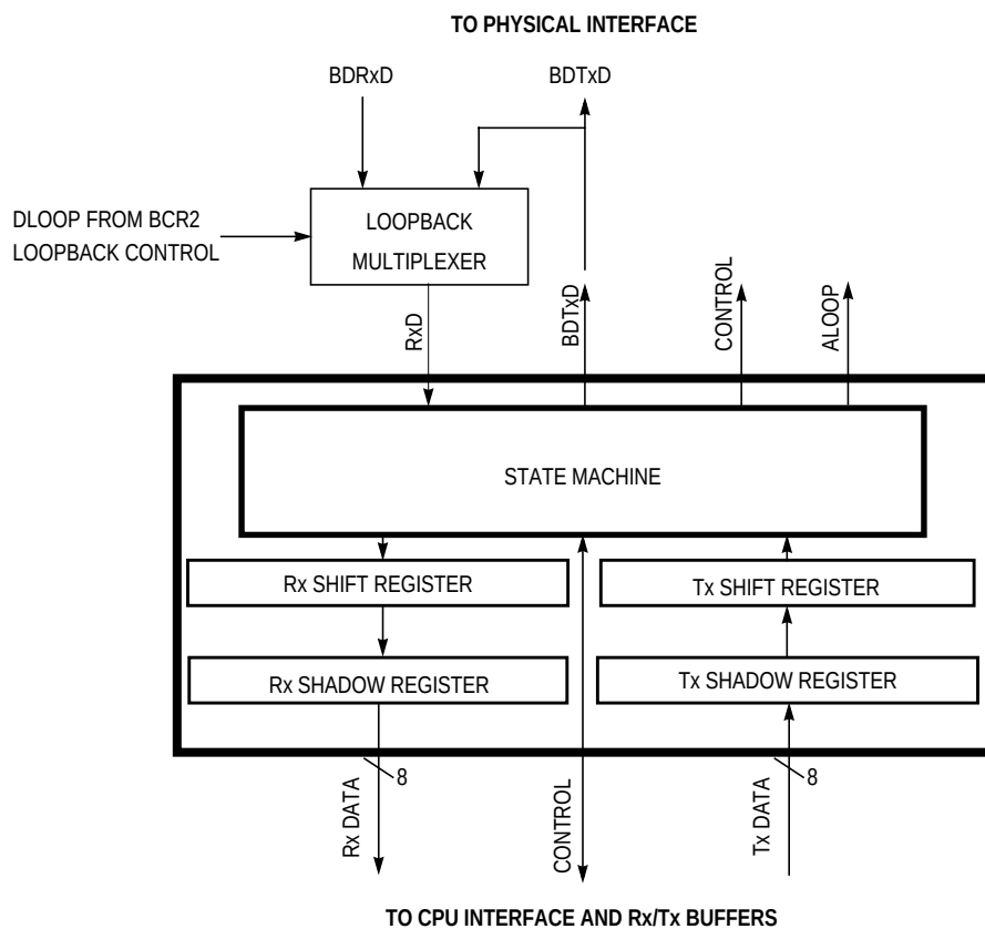
Figure 20-13. BDLC Protocol Handler Outline
