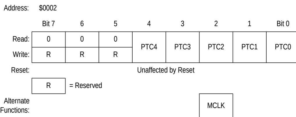
Figure 15-7. Port C Data Register (PTC)
