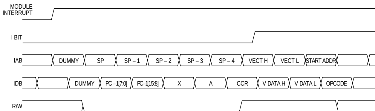
Figure 9-7. Hardware Interrupt Entry
