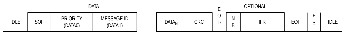
Figure 20-5. J1850 Bus Message Format (VPW)
