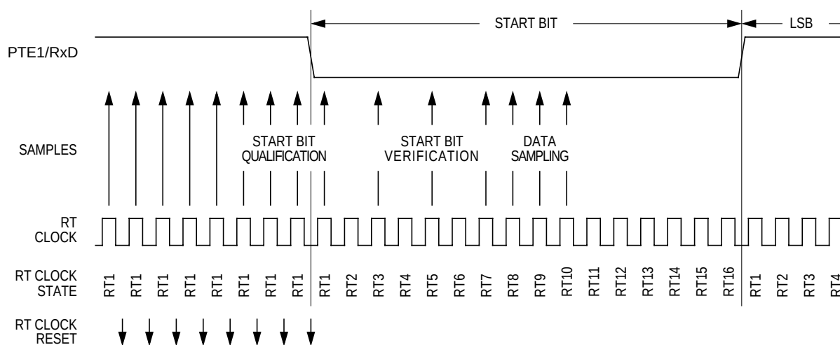
Figure 17-5. Receiver Data Sampling
