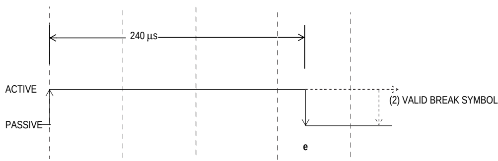
Figure 20-10. J1850 VPW Received BREAK Symbol Times
