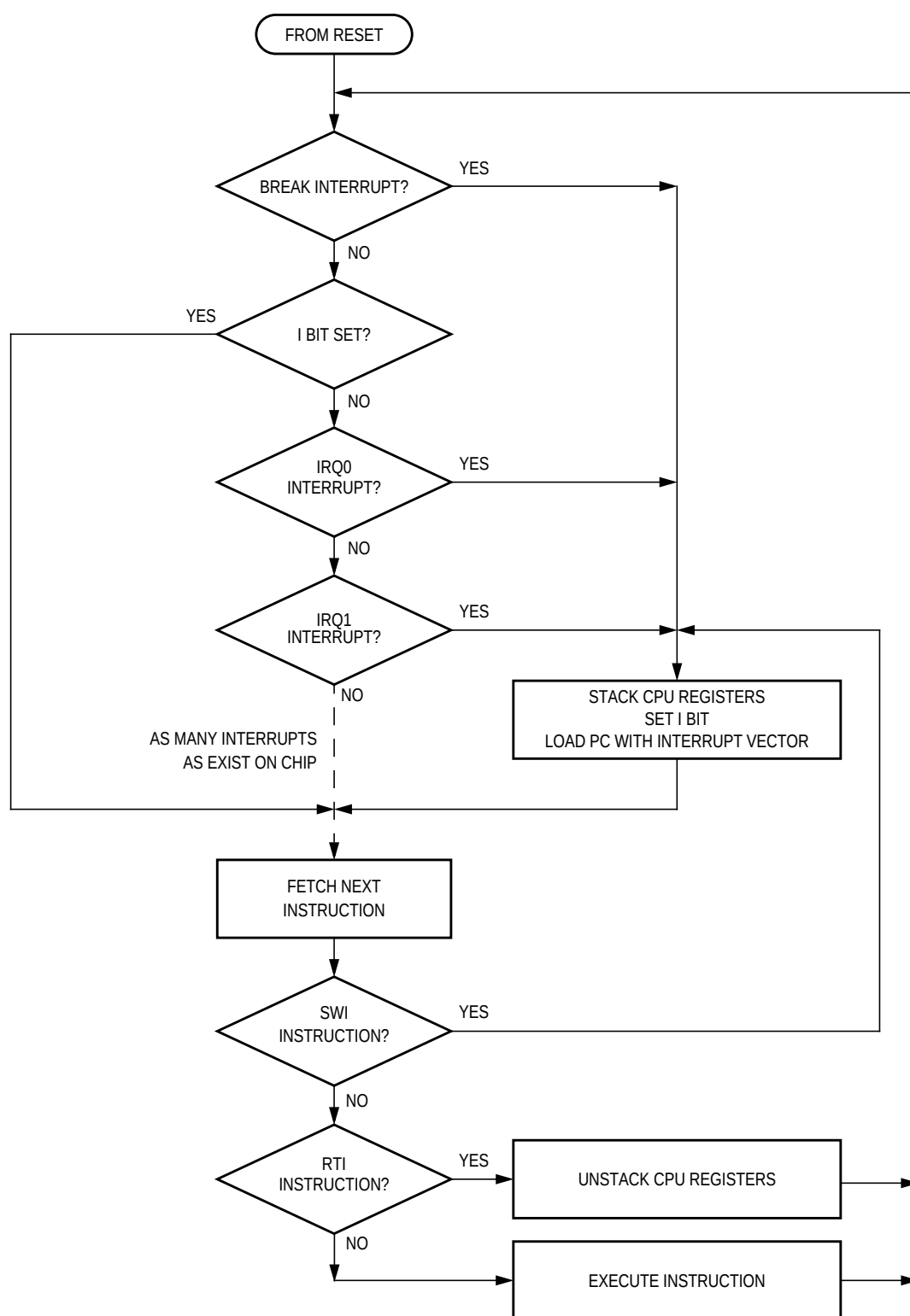
Figure 9-8. Interrupt Processing
