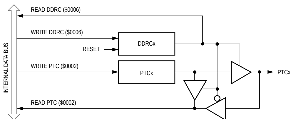
Figure 15-9. Port C I/O Circuit
