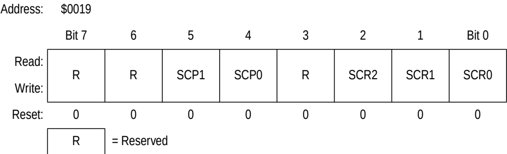
Figure 17-13. SCI BAUD Rate Register 1 (SCBR)
