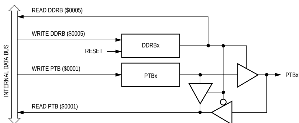
Figure 15-6. Port B I/O Circuit
