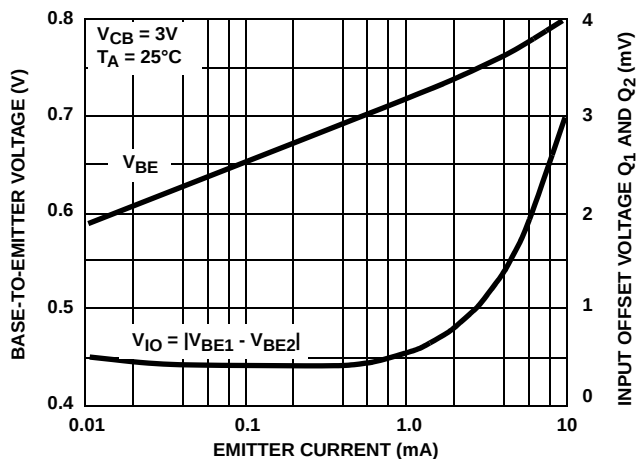
FIGURE 8. STATIC BASE-TO-EMITTER VOLTAGE AND INPUT OFFSET VOLTAGE FOR DIFFERENTIAL PAIRS vs EMITTER CURRENT
