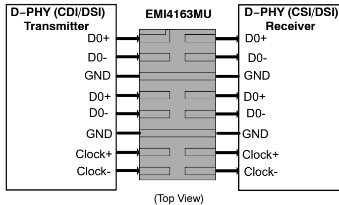
Figure 18. EMI4163MU MIPI D-PHY Application Diagram
