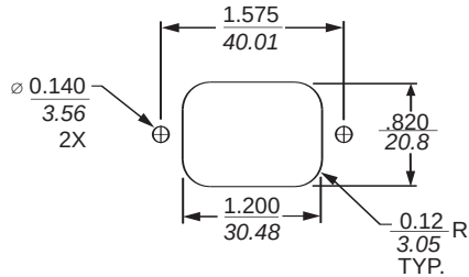
Front Mount
