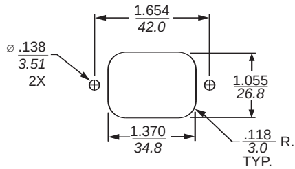
Front Mount
