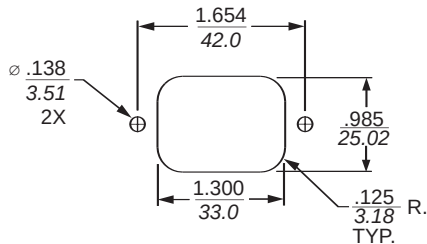
Back Mount
