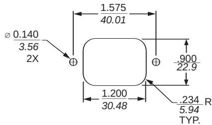
Back Mount
