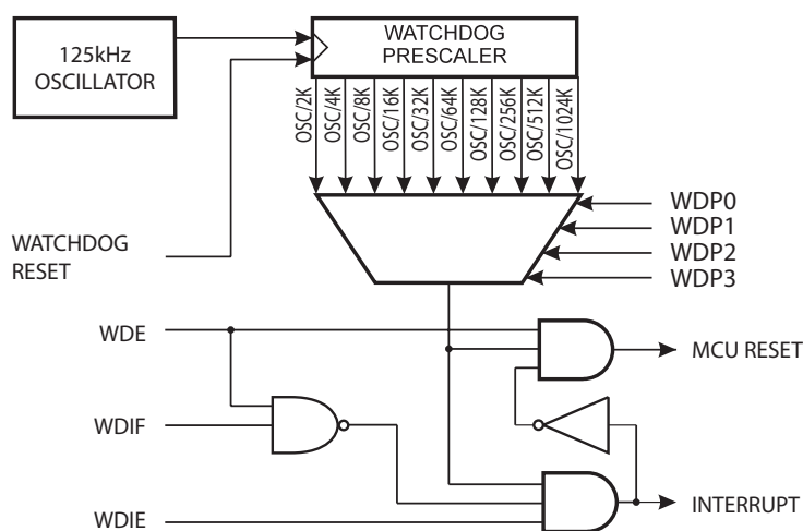
Figure 9-8. Watchdog Timer
