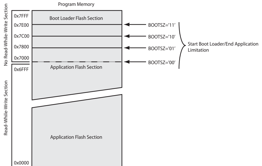
Figure 28-2. Memory Sections
