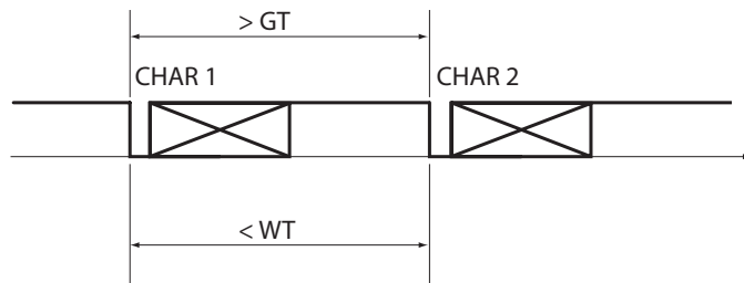
Figure 15-6. T=0 mode
