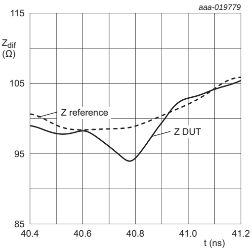
Fig 4. Differential Time Domain Reflectometer (TDR) plot; typical values
