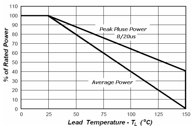
Fig3. Power Derating
