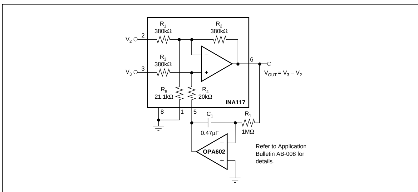
FIGURE 16. AC-Coupled INA117.
