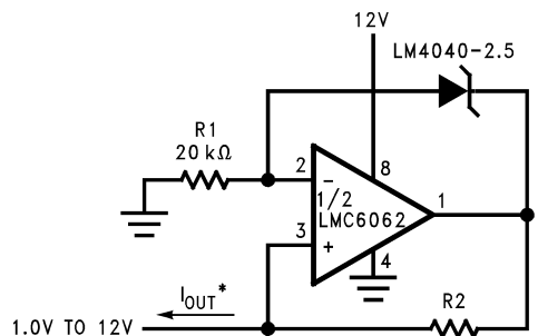
Figure 17. Precision 1-mA Current Source
