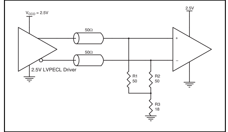
Figure 5B. 2.5V LVPECL Driver Termination Example
