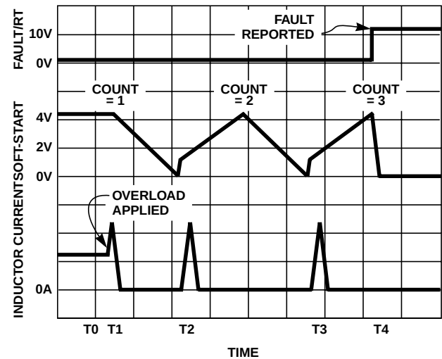
FIGURE 8. OVER-CURRENT OPERATION
