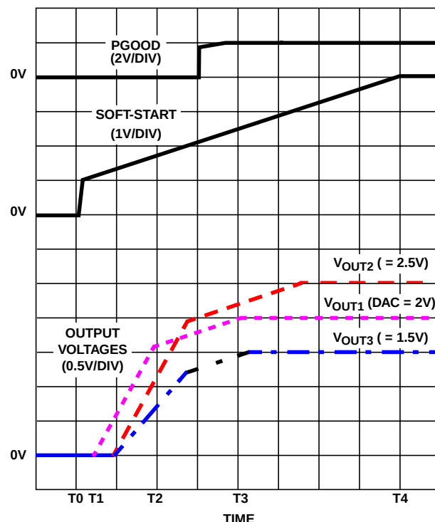
FIGURE 6. SOFT-START INTERVAL
