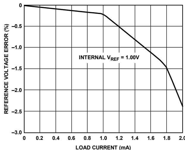
Figure 49. V_{REF} Accuracy vs. Load Current
