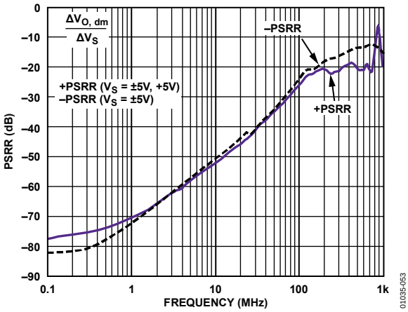
Figure 46. PSRR vs. Frequency
