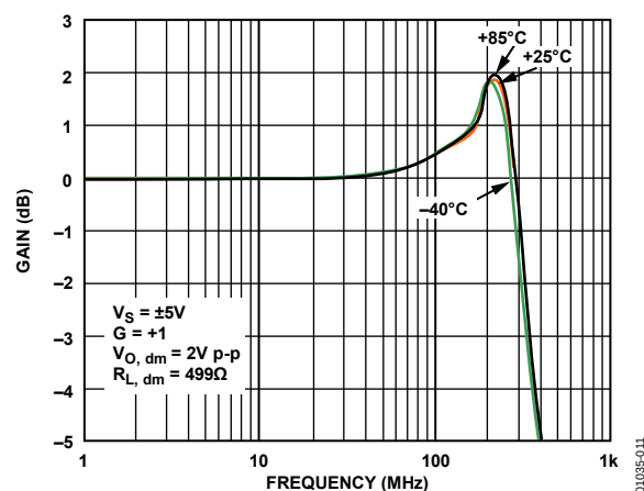
Figure 10. Large Signal Frequency Response at Various Temperatures (See Figure 56)
