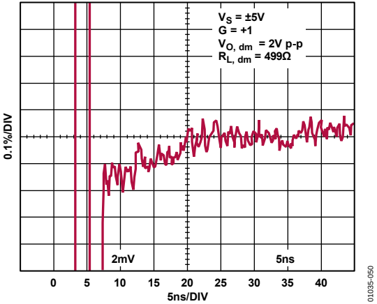
Figure 44. 0.1% Settling Time
