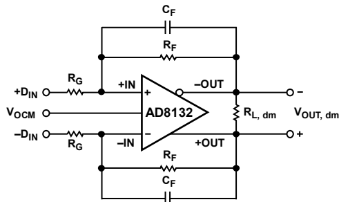
Figure 64. Circuit Definitions
