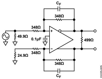
Figure 56. Basic Test Circuit, G = +1
