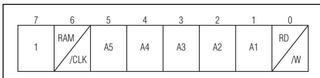
Figure 24. Address/Command Byte
