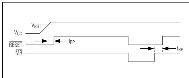
Figure 7. Manual Reset Timing
