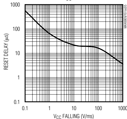
RESET COMPARATOR DELAY vs. V_{CC} FALLING
